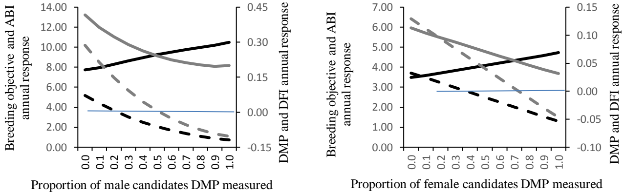
Figure 2 Annual response (per head per year) in males (left) and females (right) in combined breeding objective (BO: $, black, solid line), Angus Breeding Index (ABI: $, grey, solid), daily methane production (DMP: kg CO 2 e/d, black, dashed), and daily feed intake (DFI: kg/d, grey, dashed) versus the proportion of candidates measured for DMP. Average generation length (3.4 years) was used, so the total response is the average of the male and female responses.
